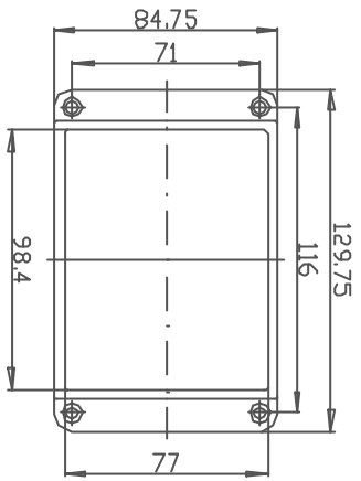
Deckel
